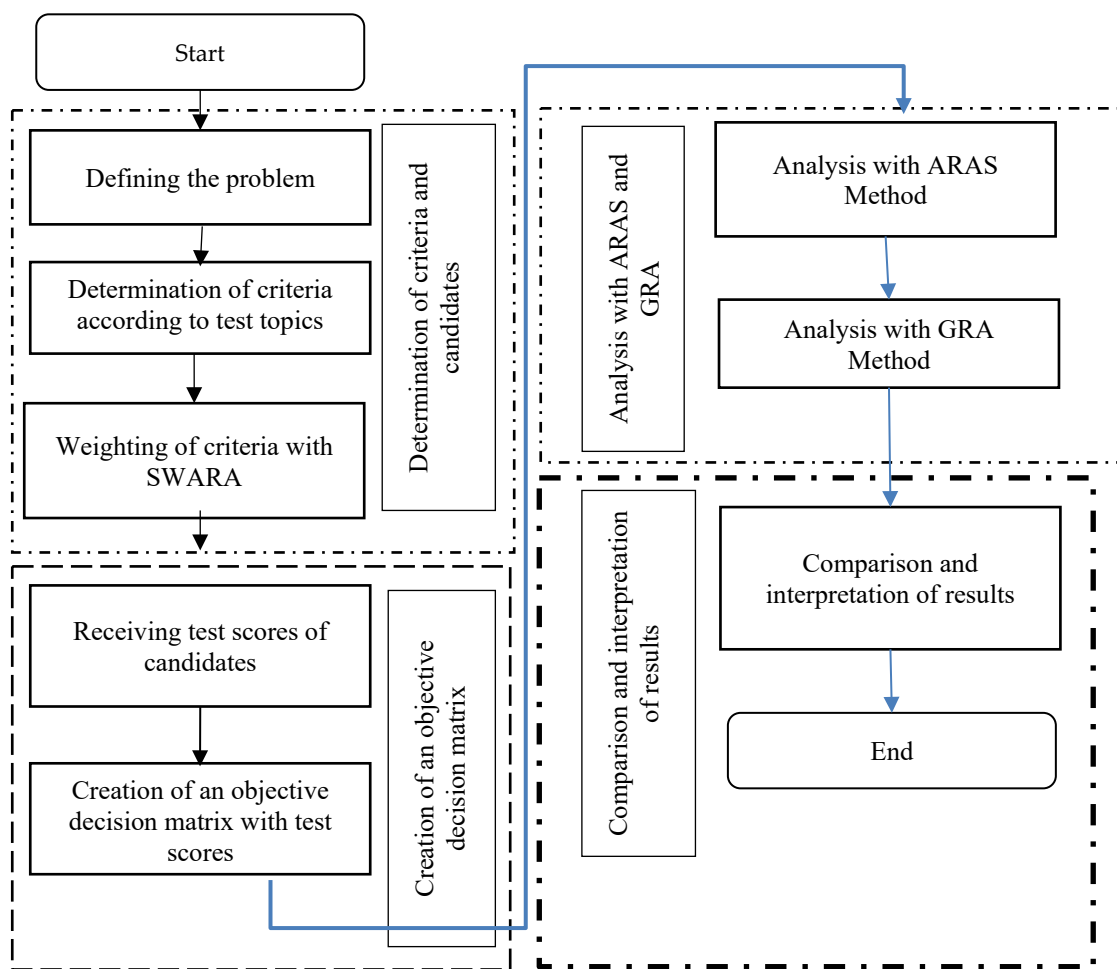
Figure 1: Proposed Model
